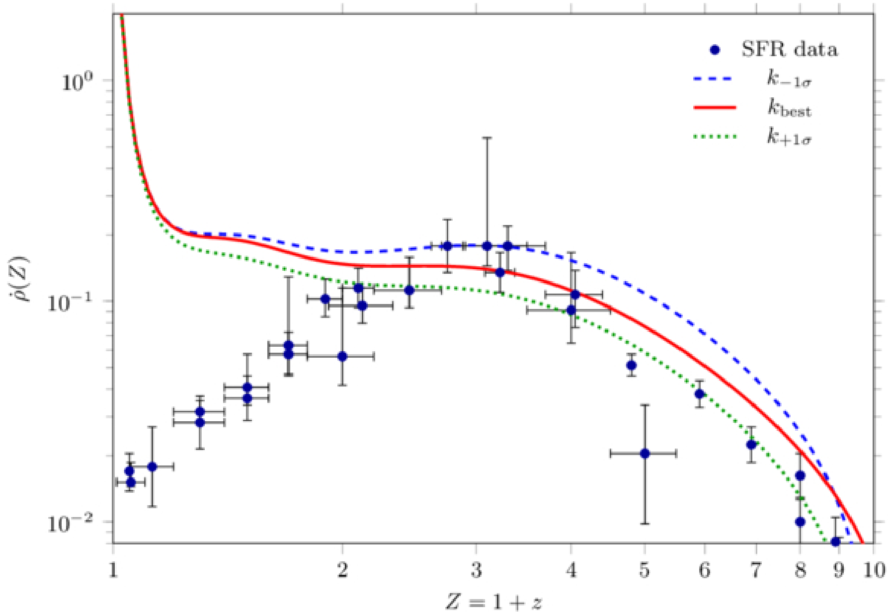
Figure 10. from Sujay Champati et al 2026 Astrophys. J. 1005 doi:10.3847/1538-4357/ae77e2 https://dx.doi.org/10.3847/1538-4357/ae77e2 © 2026. The Author(s). Published by the American Astronomical Society.
