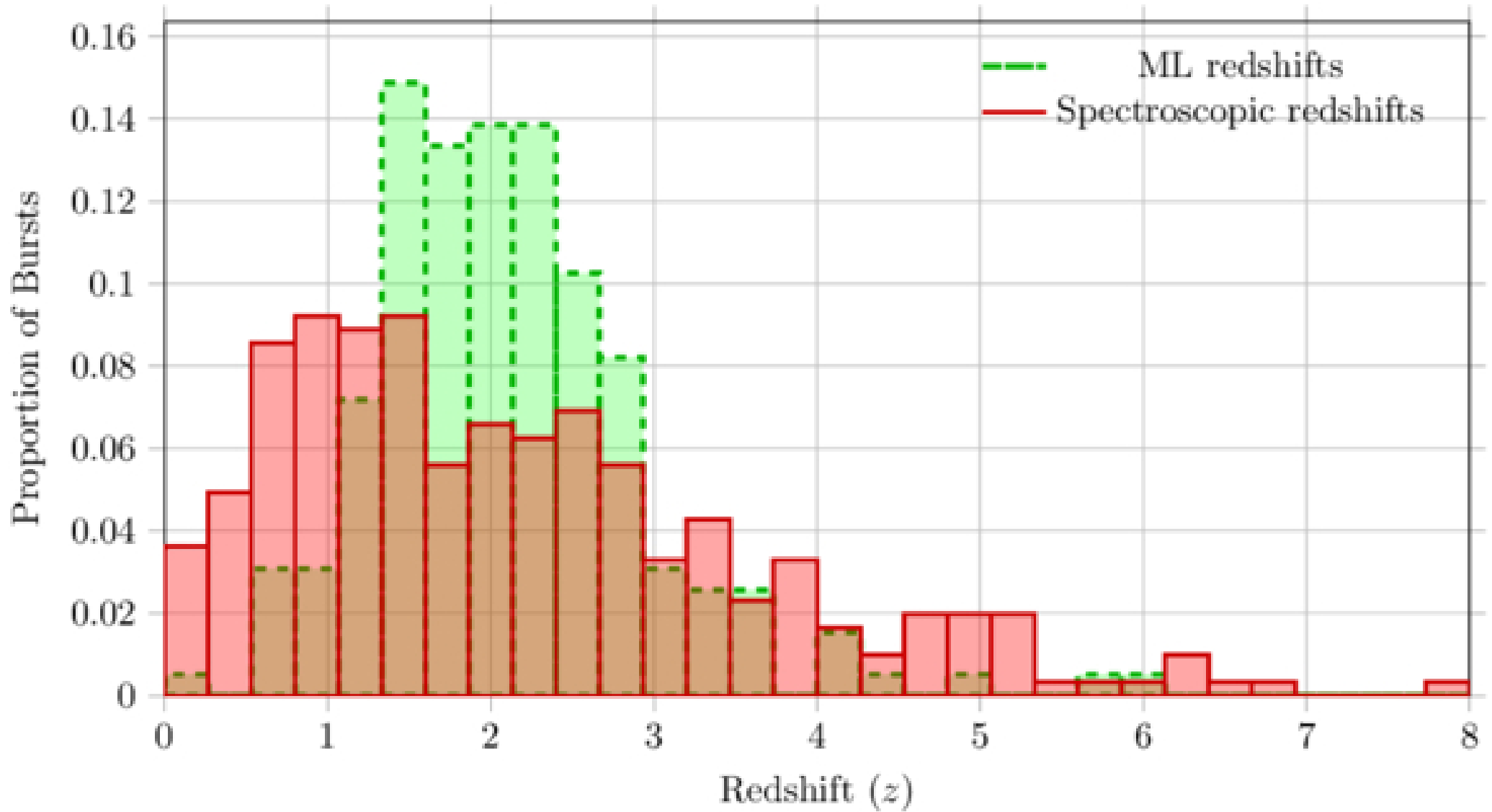
Figure 1. from Sujay Champati et al 2026 Astrophys. J. 1005 doi:10.3847/1538-4357/ae77e2 https://dx.doi.org/10.3847/1538-4357/ae77e2 © 2026. The Author(s). Published by the American Astronomical Society.
