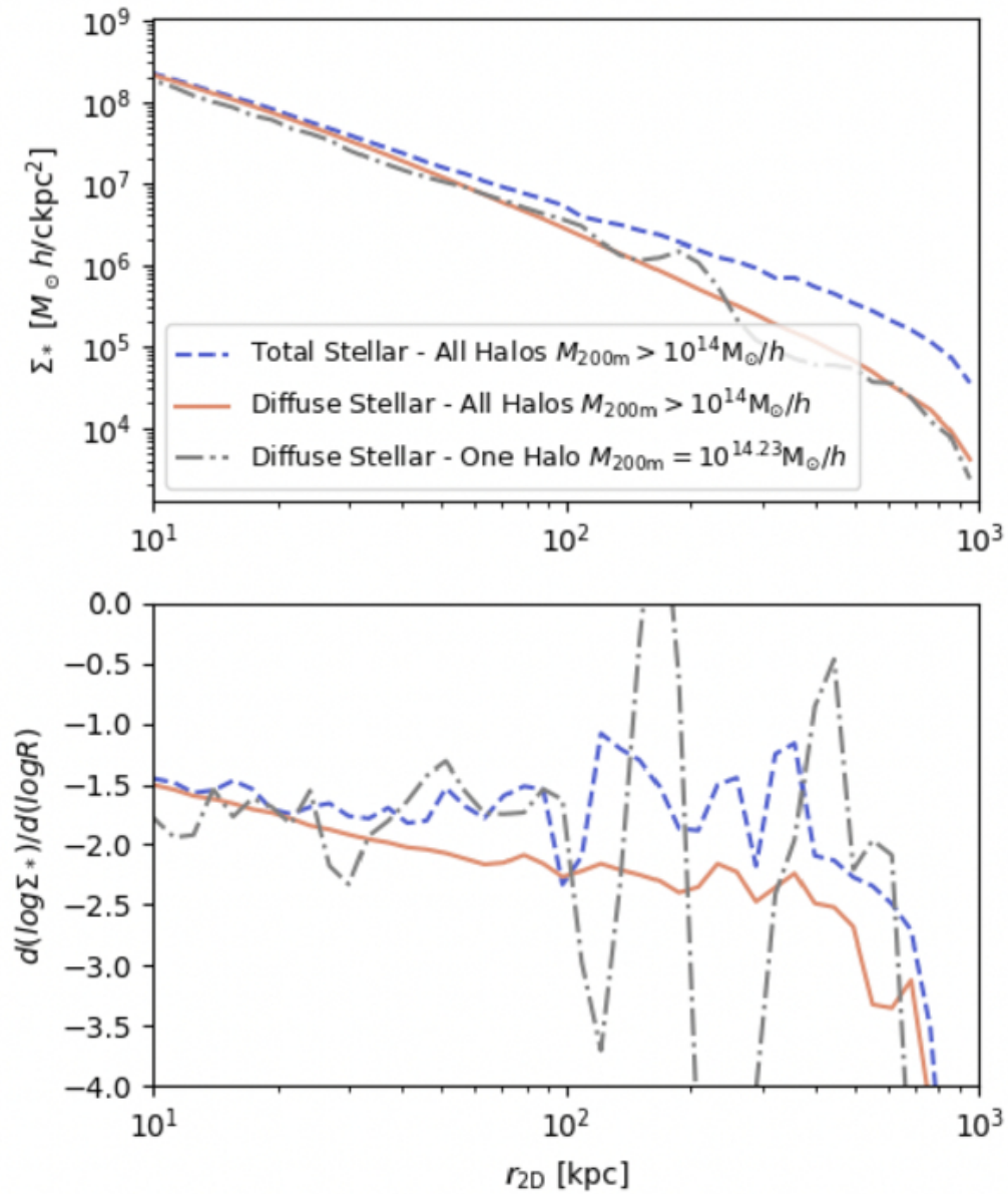
Figure 8. from Yuanyuan Zhang et al 2026 Astrophys. J. 1006 doi:10.3847/1538-4357/ae76d1 https://dx.doi.org/10.3847/1538-4357/ae76d1 © 2026. The Author(s). Published by the American Astronomical Society.
