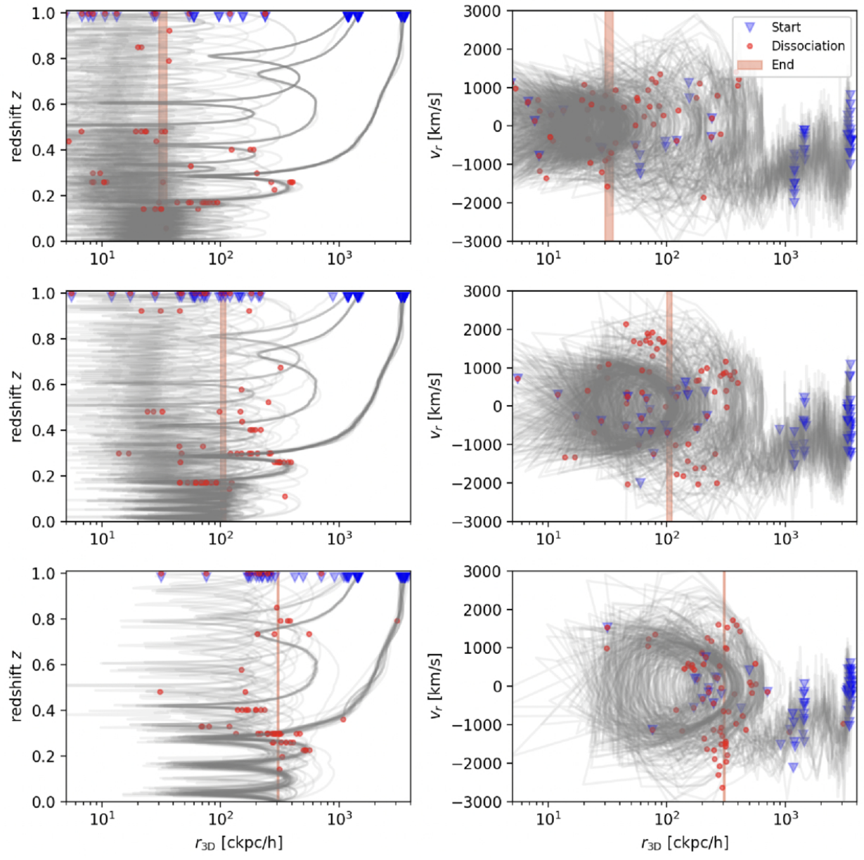
Figure 6. from Yuanyuan Zhang et al 2026 Astrophys. J. 1006 doi:10.3847/1538-4357/ae76d1 https://dx.doi.org/10.3847/1538-4357/ae76d1 © 2026. The Author(s). Published by the American Astronomical Society.
