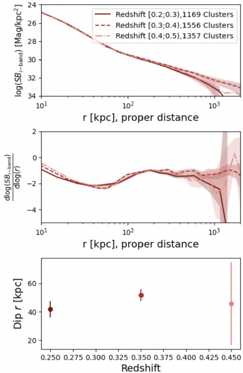
Figure 1. from Yuanyuan Zhang et al 2026 Astrophys. J. 1006 doi:10.3847/1538-4357/ae76d1 https://dx.doi.org/10.3847/1538-4357/ae76d1 © 2026. The Author(s). Published by the American Astronomical Society.
