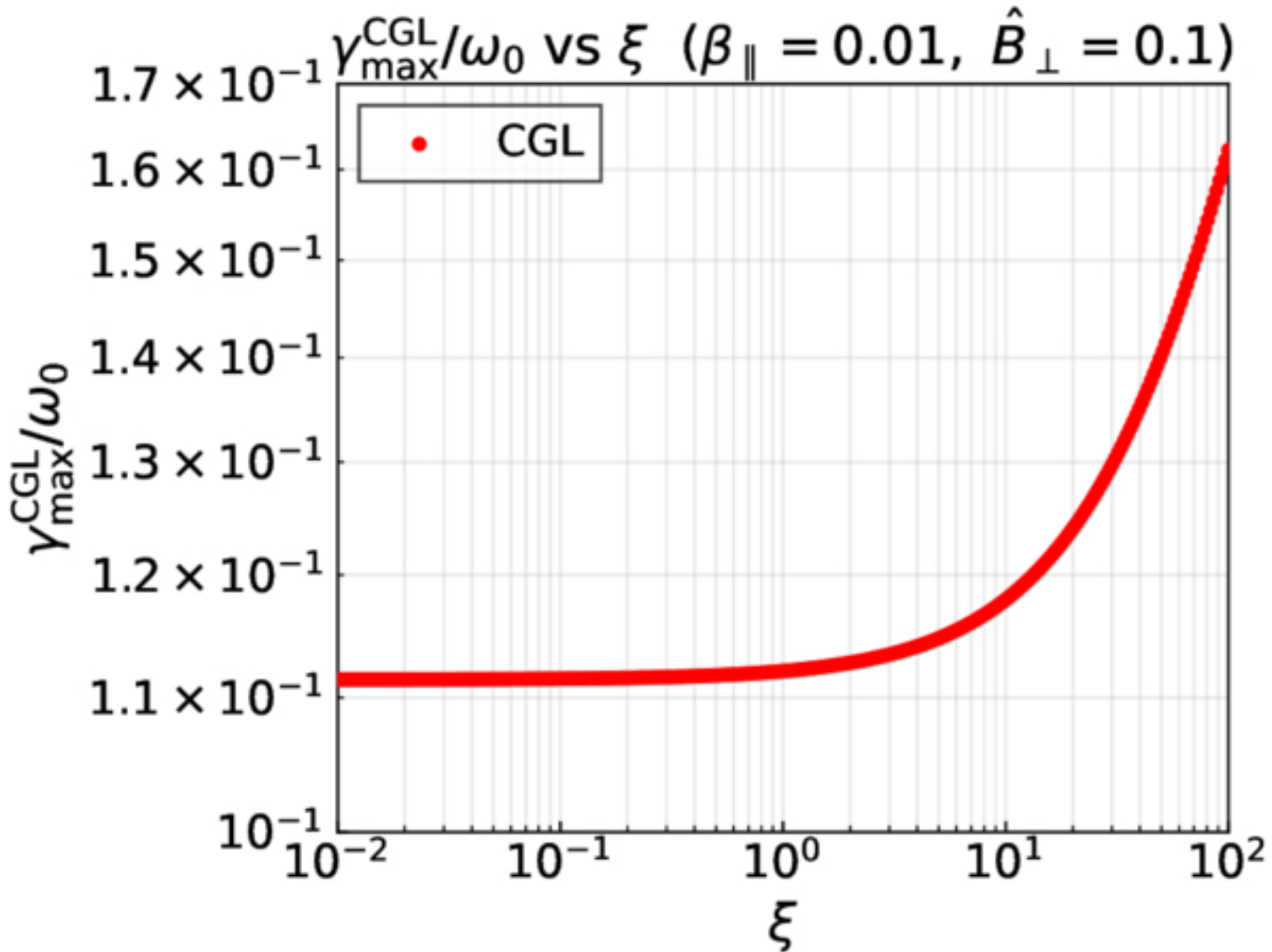
Figure 7. from Hayato Saguchi et al 2026 Astrophys. J. 1005 doi:10.3847/1538-4357/ae7699 https://dx.doi.org/10.3847/1538-4357/ae7699 © 2026. The Author(s). Published by the American Astronomical Society.
