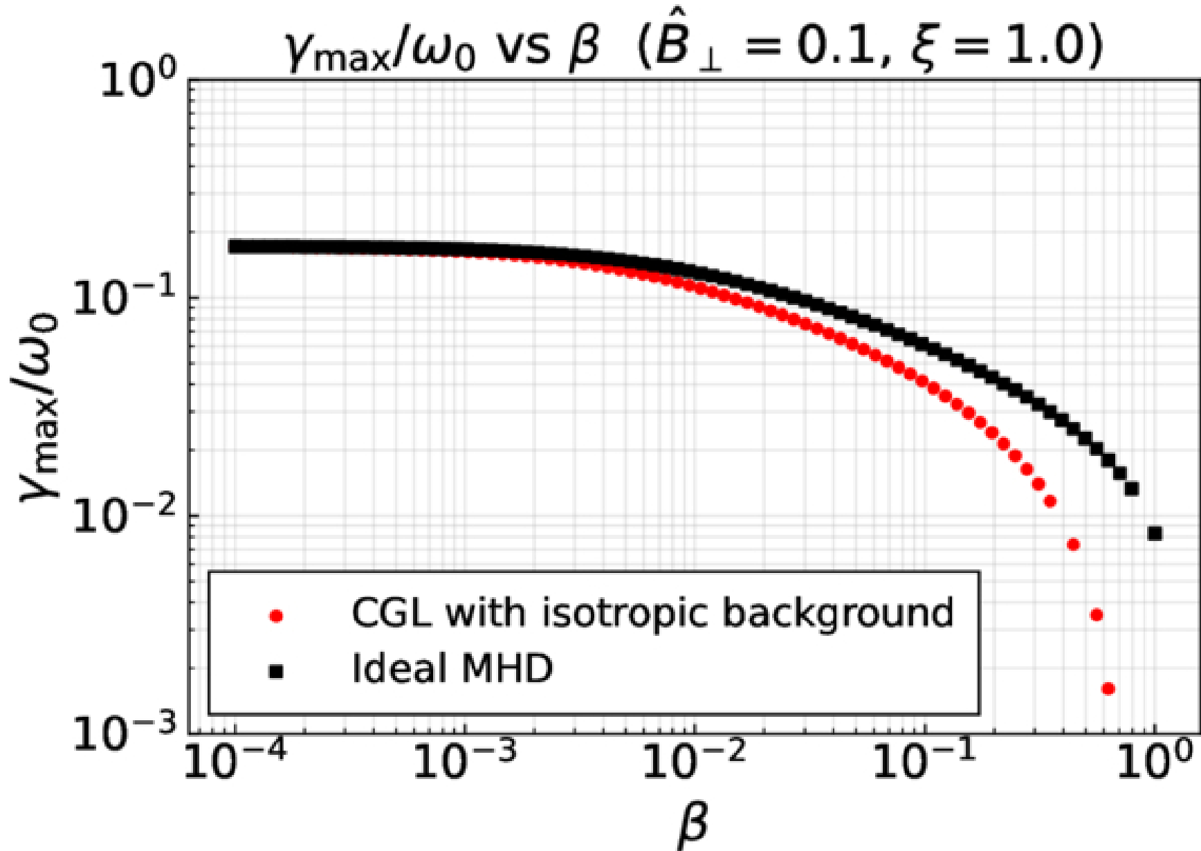
Figure 5. from Hayato Saguchi et al 2026 Astrophys. J. 1005 doi:10.3847/1538-4357/ae7699 https://dx.doi.org/10.3847/1538-4357/ae7699 © 2026. The Author(s). Published by the American Astronomical Society.
