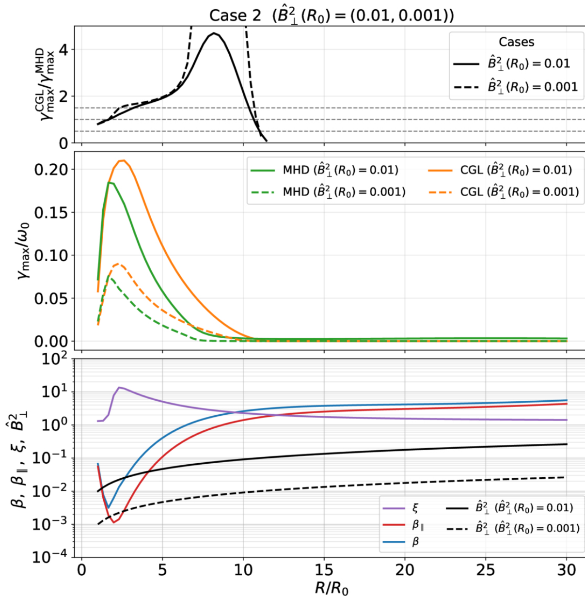
Figure 3. from Hayato Saguchi et al 2026 Astrophys. J. 1005 doi:10.3847/1538-4357/ae7699 https://dx.doi.org/10.3847/1538-4357/ae7699 © 2026. The Author(s). Published by the American Astronomical Society.
