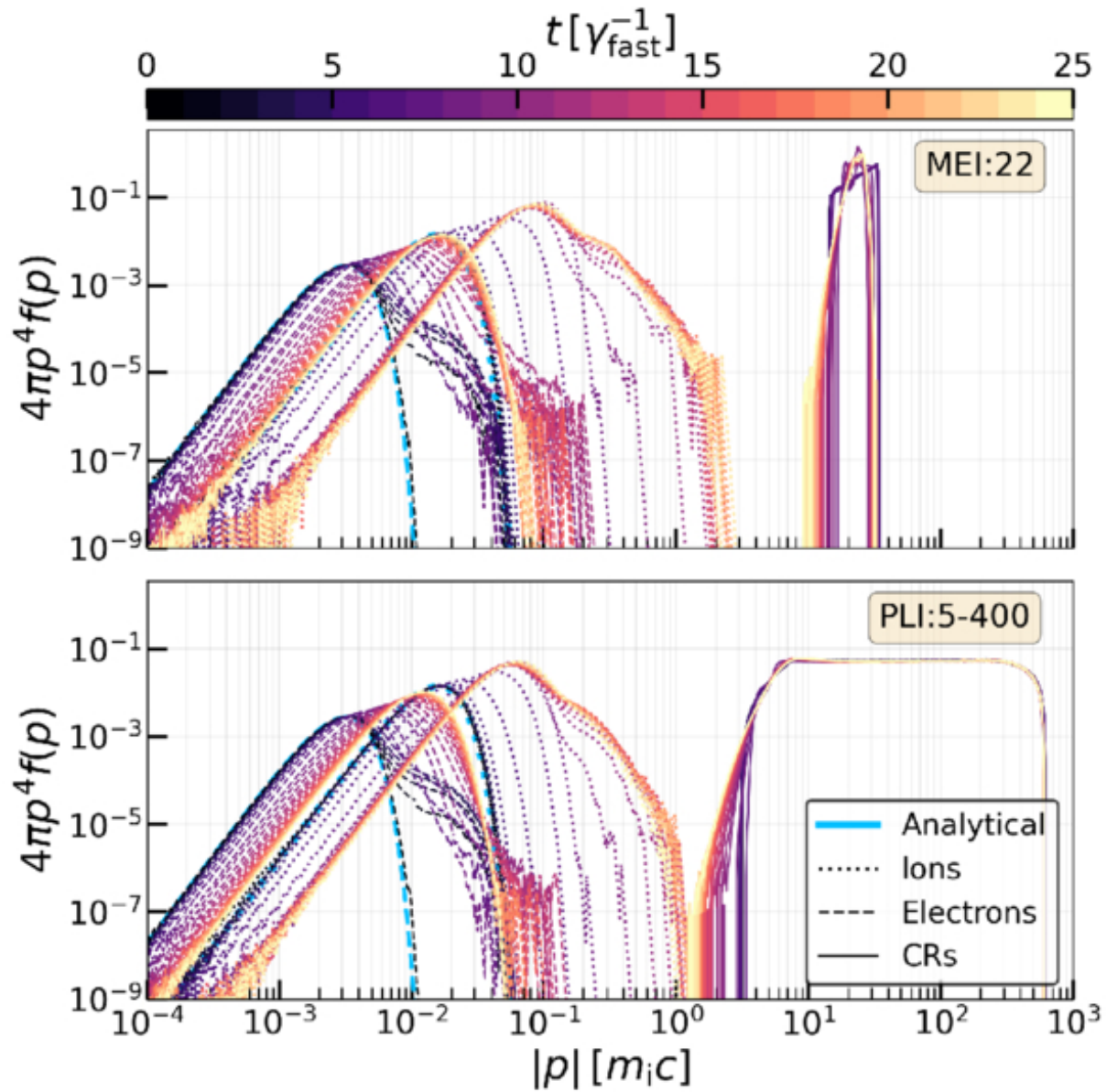
Figure 6. from Saikat Das et al 2026 Astrophys. J. 1005 doi:10.3847/1538-4357/ae75ff https://dx.doi.org/10.3847/1538-4357/ae75ff © 2026. The Author(s). Published by the American Astronomical Society.
