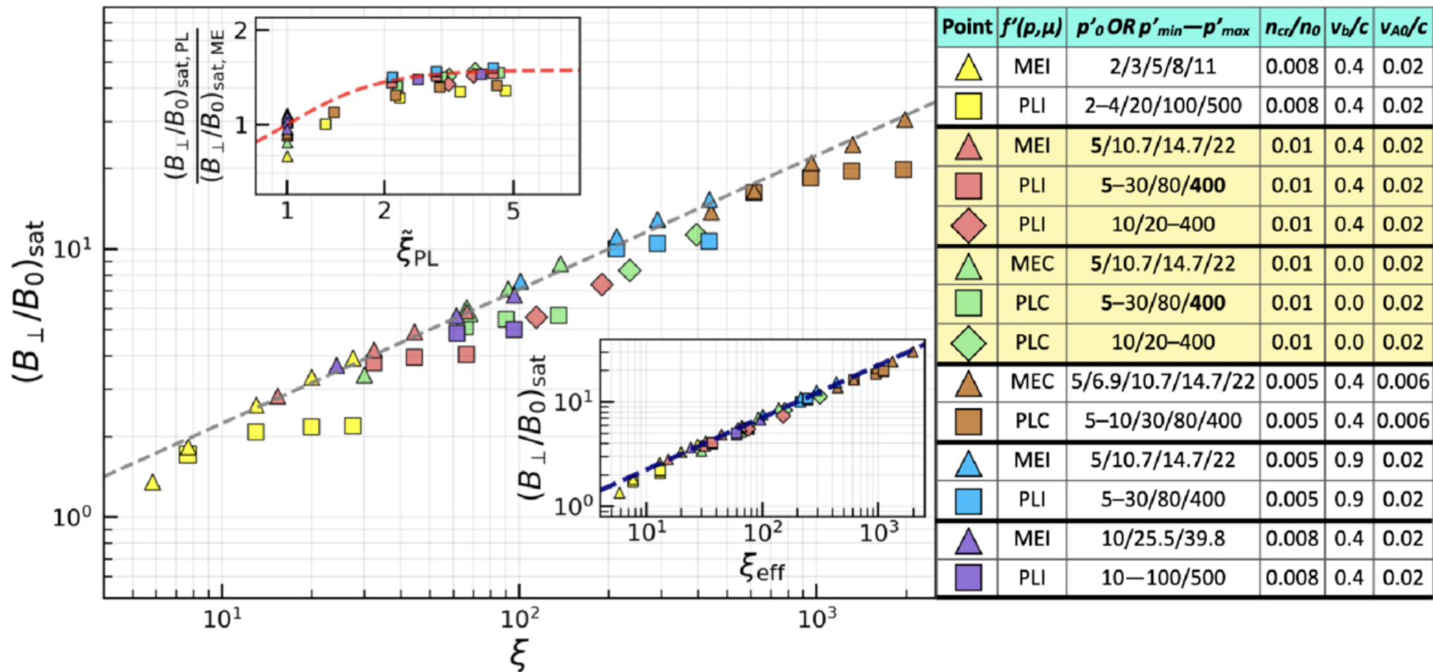
Figure 5. from Saikat Das et al 2026 Astrophys. J. 1005 doi:10.3847/1538-4357/ae75ff https://dx.doi.org/10.3847/1538-4357/ae75ff © 2026. The Author(s). Published by the American Astronomical Society.
