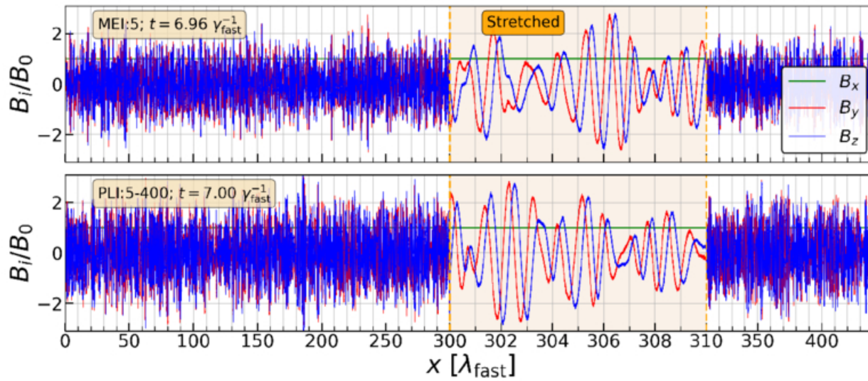
Figure 2. from Saikat Das et al 2026 Astrophys. J. 1005 doi:10.3847/1538-4357/ae75ff https://dx.doi.org/10.3847/1538-4357/ae75ff © 2026. The Author(s). Published by the American Astronomical Society.
