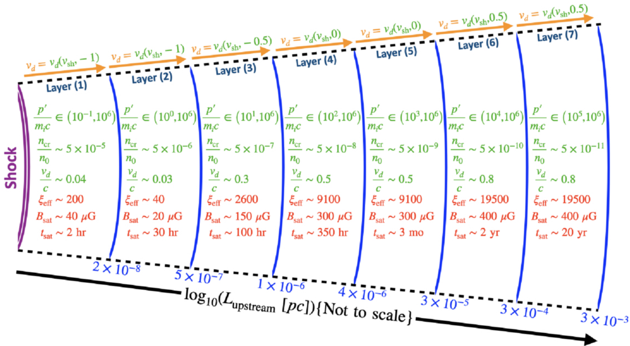
Figure 10. from Saikat Das et al 2026 Astrophys. J. 1005 doi:10.3847/1538-4357/ae75ff https://dx.doi.org/10.3847/1538-4357/ae75ff © 2026. The Author(s). Published by the American Astronomical Society.
