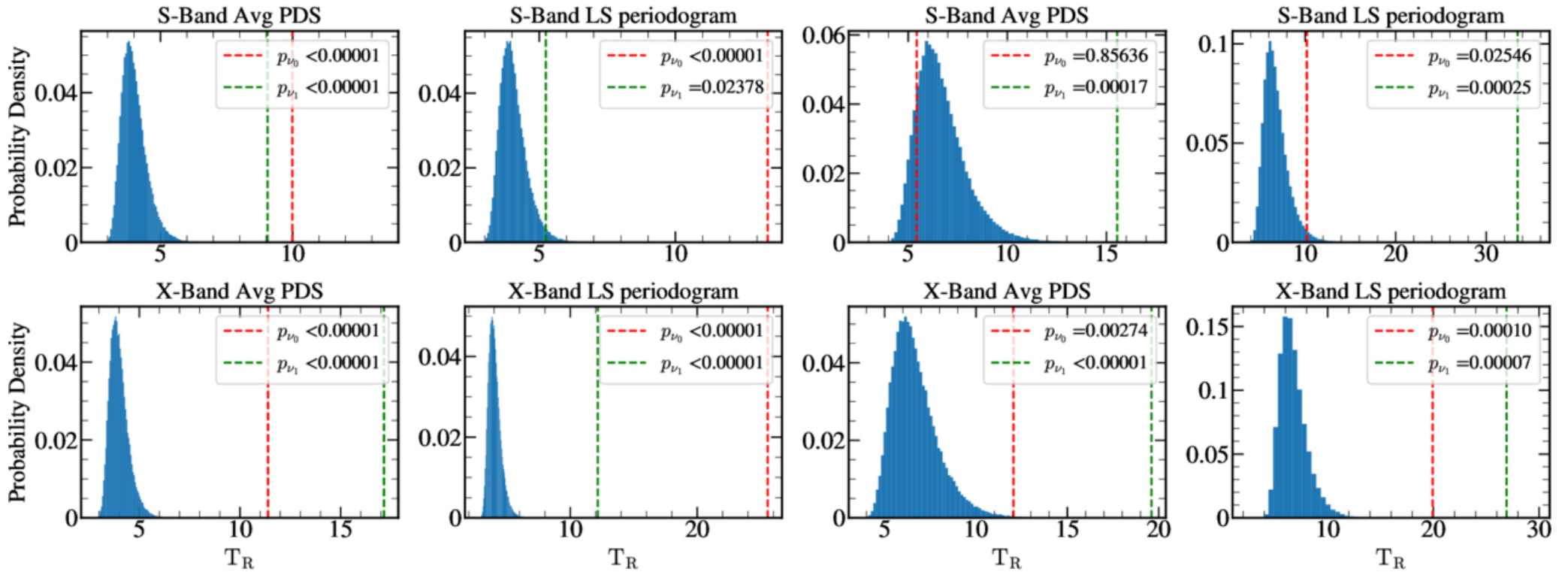
Figure 3. from Ya Xing Li et al 2026 Astrophys. J. 1004 doi:10.3847/1538-4357/ae75a5 https://dx.doi.org/10.3847/1538-4357/ae75a5 © 2026. The Author(s). Published by the American Astronomical Society.
