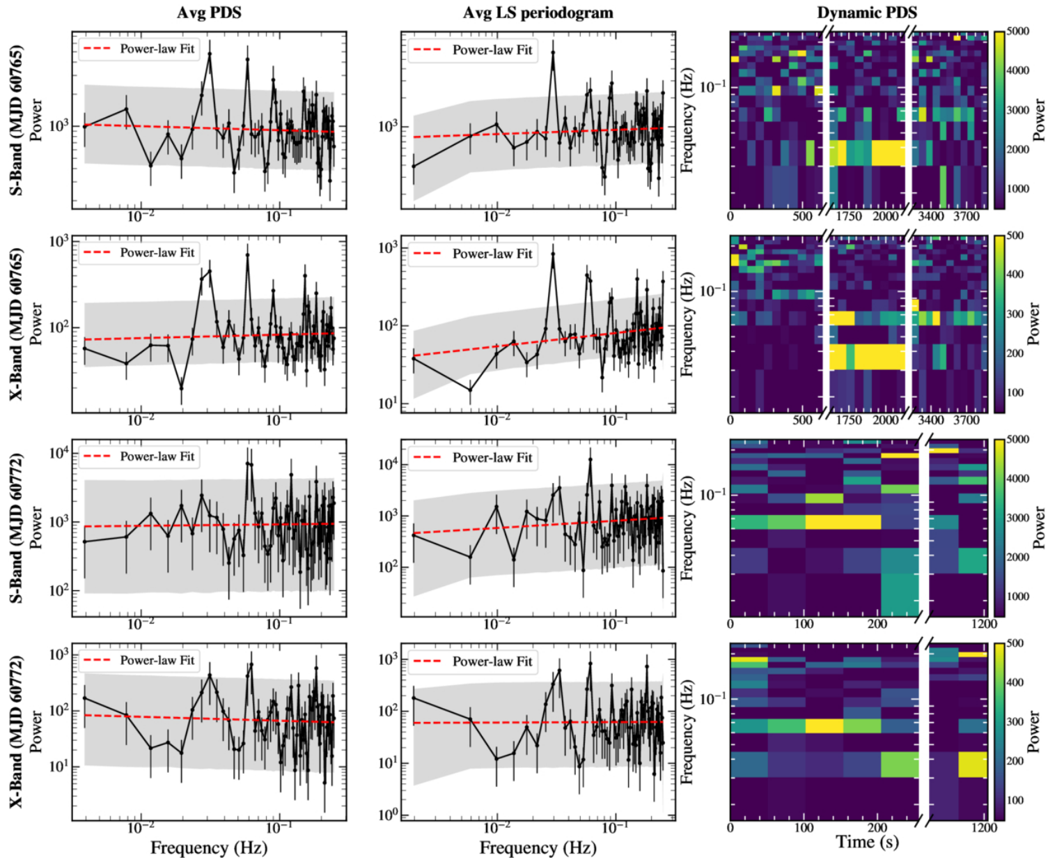
Figure 2. from Ya Xing Li et al 2026 Astrophys. J. 1004 doi:10.3847/1538-4357/ae75a5 https://dx.doi.org/10.3847/1538-4357/ae75a5 © 2026. The Author(s). Published by the American Astronomical Society.
