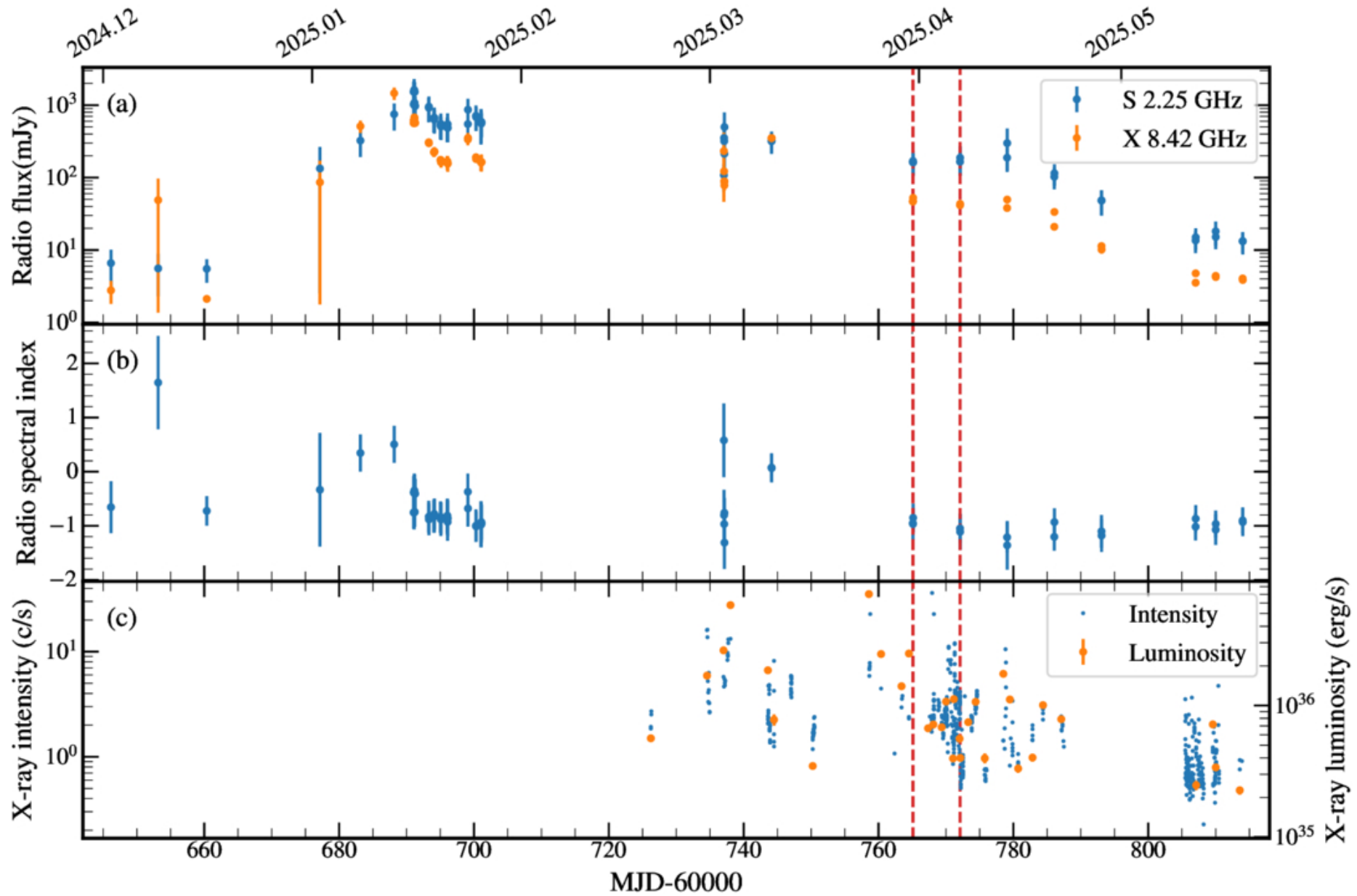
Figure 1. from Ya Xing Li et al 2026 Astrophys. J. 1004 doi:10.3847/1538-4357/ae75a5 https://dx.doi.org/10.3847/1538-4357/ae75a5 © 2026. The Author(s). Published by the American Astronomical Society.
