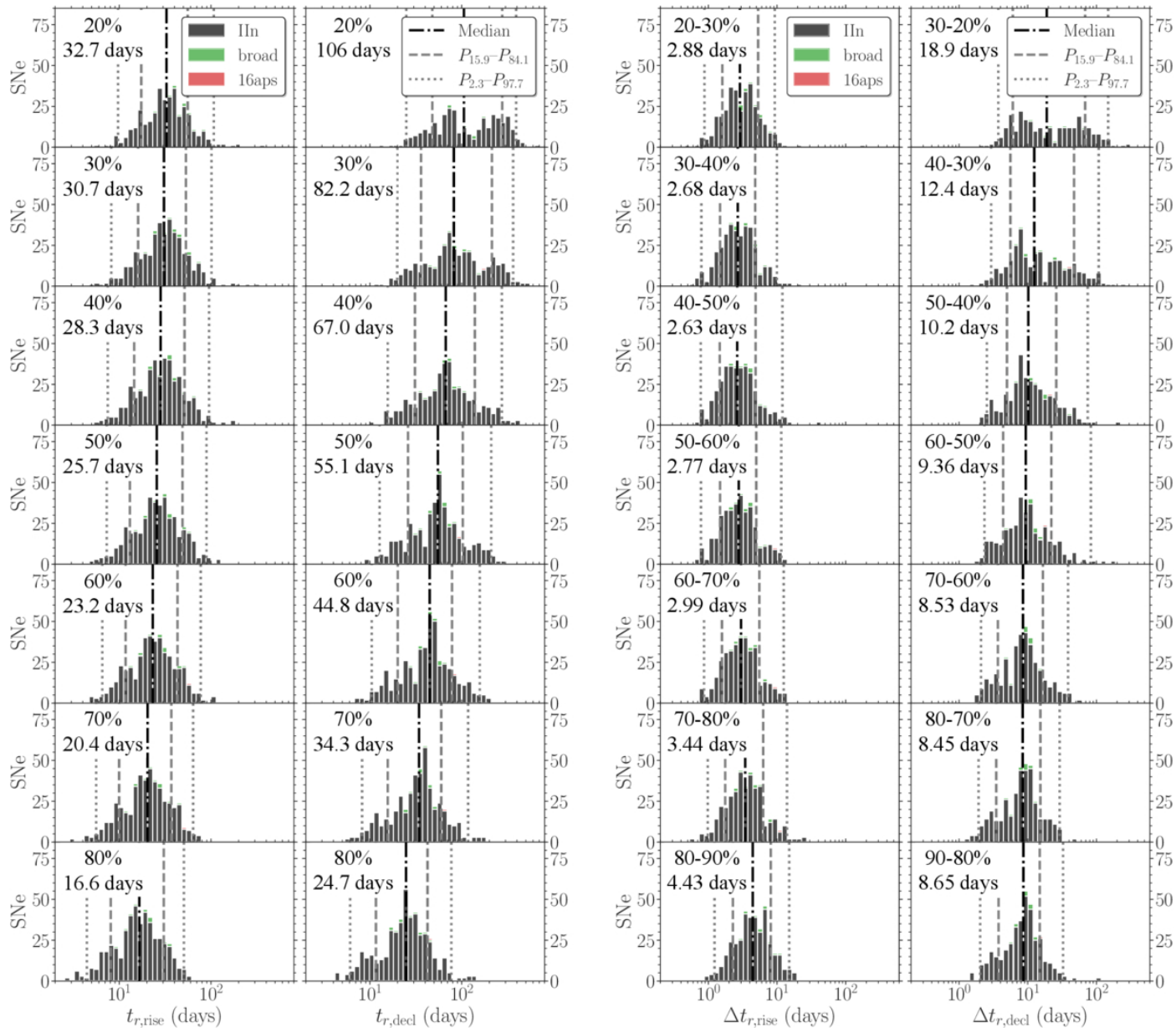
Figure 9. from Daichi Hiramatsu et al 2026 Astrophys. J. 1005 doi:10.3847/1538-4357/ae743c https://dx.doi.org/10.3847/1538-4357/ae743c © 2026. The Author(s). Published by the American Astronomical Society.
