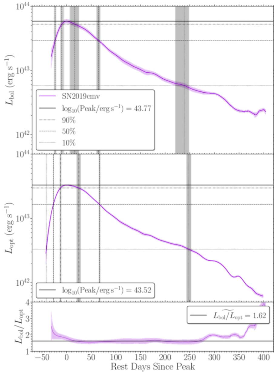
Figure 3. from Daichi Hiramatsu et al 2026 Astrophys. J. 1005 doi:10.3847/1538-4357/ae743c https://dx.doi.org/10.3847/1538-4357/ae743c © 2026. The Author(s). Published by the American Astronomical Society.
