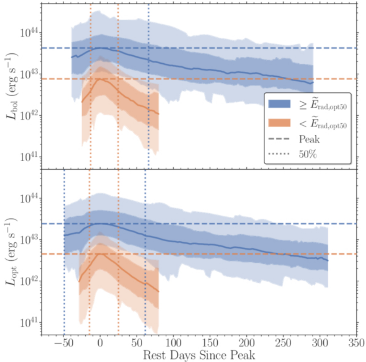
Figure 19. from Daichi Hiramatsu et al 2026 Astrophys. J. 1005 doi:10.3847/1538-4357/ae743c https://dx.doi.org/10.3847/1538-4357/ae743c © 2026. The Author(s). Published by the American Astronomical Society.
