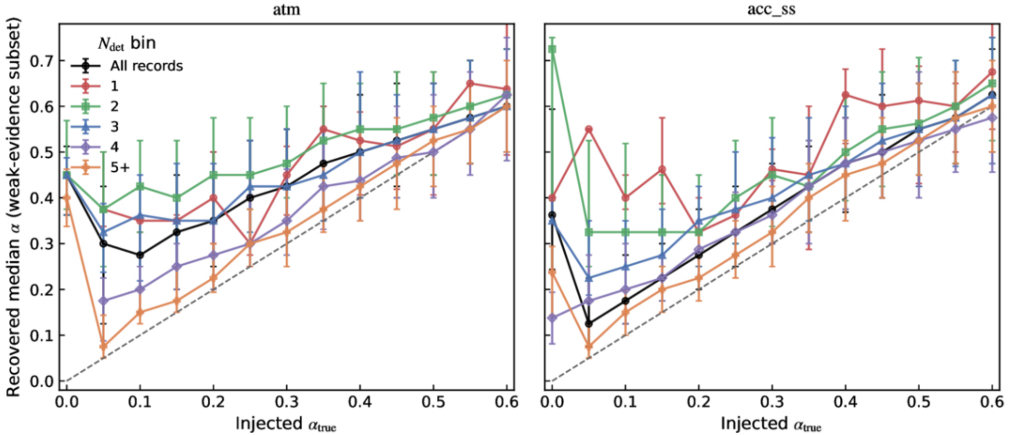
Figure 6. from Bo-Lun Huang et al 2026 Astrophys. J. 1006 doi:10.3847/1538-4357/ae742c https://dx.doi.org/10.3847/1538-4357/ae742c © 2026. The Author(s). Published by the American Astronomical Society.
