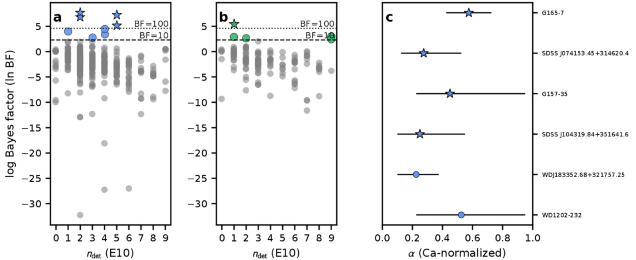
Figure 4. from Bo-Lun Huang et al 2026 Astrophys. J. 1006 doi:10.3847/1538-4357/ae742c https://dx.doi.org/10.3847/1538-4357/ae742c © 2026. The Author(s). Published by the American Astronomical Society.
