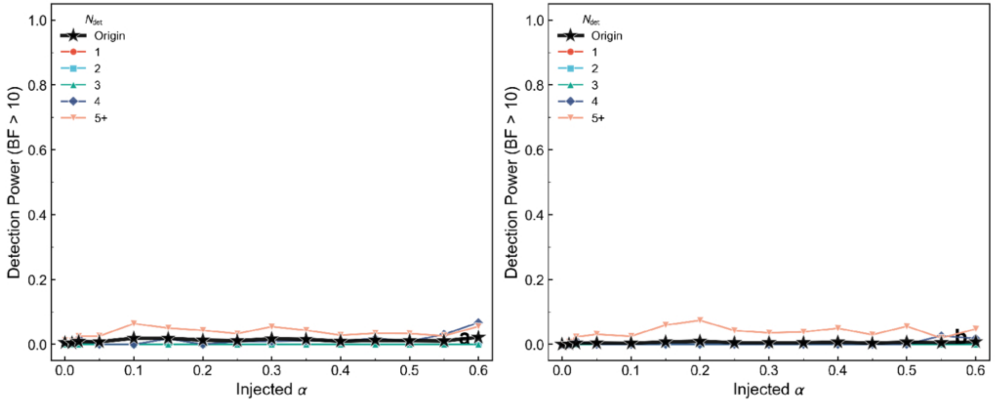
Figure A4. from Bo-Lun Huang et al 2026 Astrophys. J. 1006 doi:10.3847/1538-4357/ae742c https://dx.doi.org/10.3847/1538-4357/ae742c © 2026. The Author(s). Published by the American Astronomical Society.
