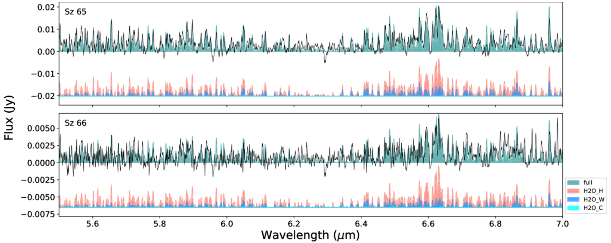
Figure 9. from Jinghui Yao et al 2026 Astrophys. J. 1005 doi:10.3847/1538-4357/ae736e https://dx.doi.org/10.3847/1538-4357/ae736e © 2026. The Author(s). Published by the American Astronomical Society.
