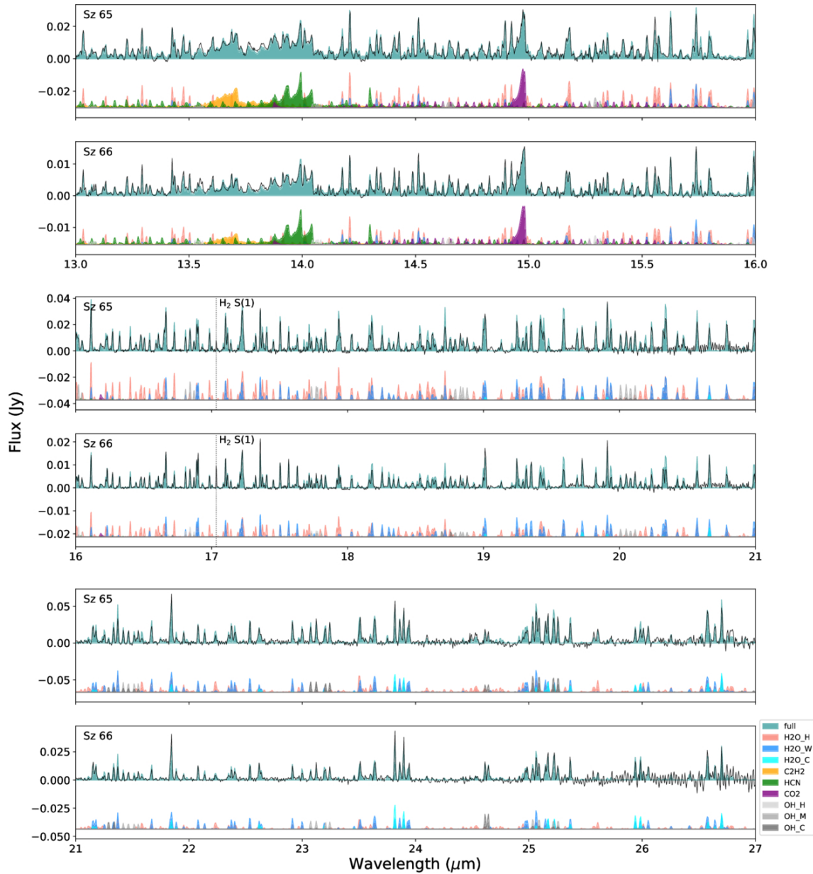
Figure 7. from Jinghuai Yao et al 2026 Astrophys. J. 1005 doi:10.3847/1538-4357/ae736e https://dx.doi.org/10.3847/1538-4357/ae736e © 2026. The Author(s). Published by the American Astronomical Society.
