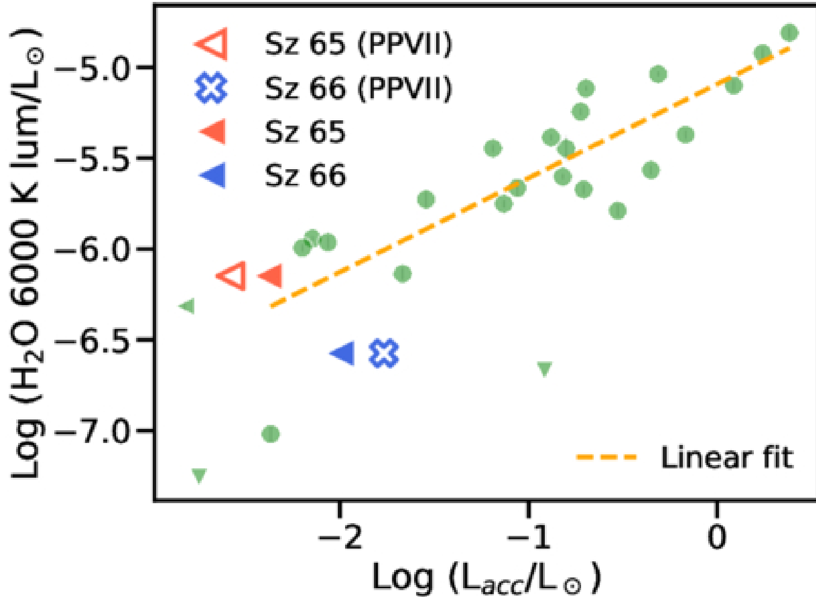
Figure 6. from Jinghui Yao et al 2026 Astrophys. J. 1005 doi:10.3847/1538-4357/ae736e https://dx.doi.org/10.3847/1538-4357/ae736e © 2026. The Author(s). Published by the American Astronomical Society.
