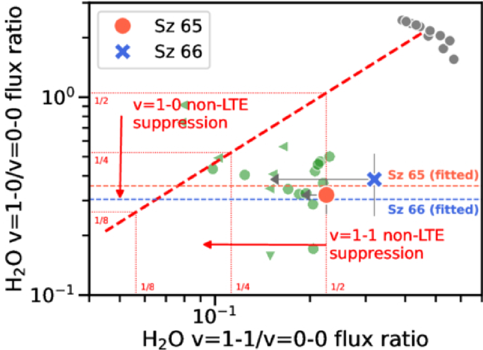
Figure 5. from Jinghui Yao et al 2026 Astrophys. J. 1005 doi:10.3847/1538-4357/ae736e https://dx.doi.org/10.3847/1538-4357/ae736e © 2026. The Author(s). Published by the American Astronomical Society.
