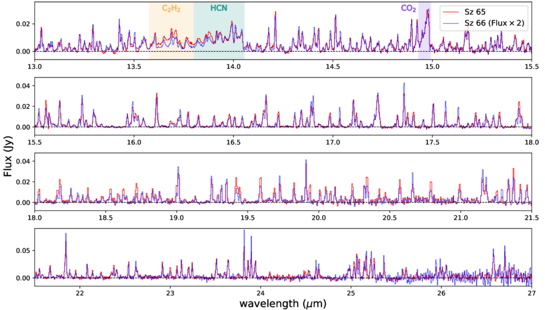
Figure 2. from Jinghui Yao et al 2026 Astrophys. J. 1005 doi:10.3847/1538-4357/ae736e https://dx.doi.org/10.3847/1538-4357/ae736e © 2026. The Author(s). Published by the American Astronomical Society.
