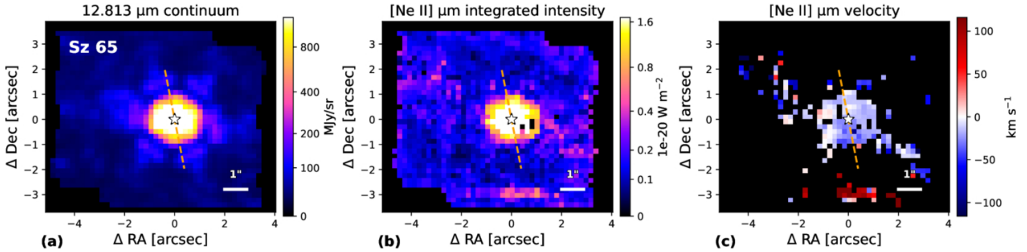
Figure 13. from Jinghuai Yao et al 2026 Astrophys. J. 1005 doi:10.3847/1538-4357/ae736e https://dx.doi.org/10.3847/1538-4357/ae736e © 2026. The Author(s). Published by the American Astronomical Society.
