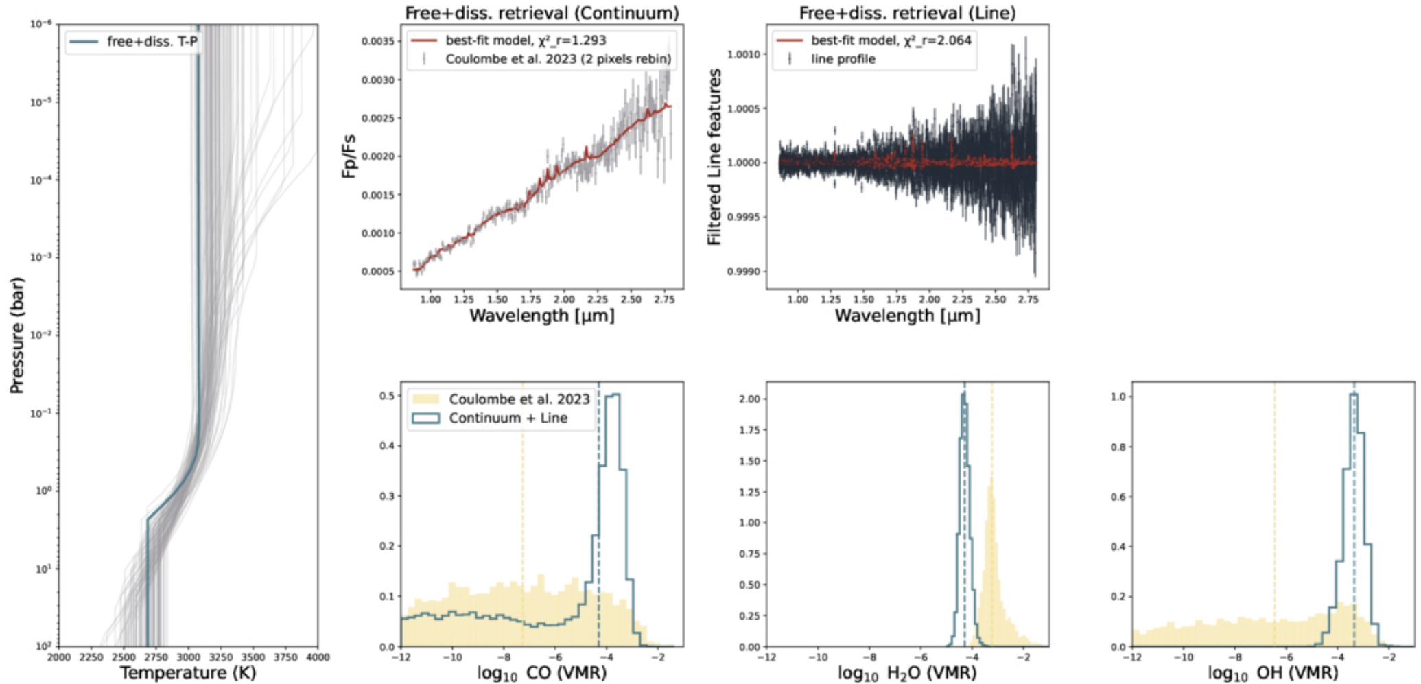
Figure 5. from Qinglin Ouyang et al 2026 Astrophys. J. 1004 doi:10.3847/1538-4357/ae736a https://dx.doi.org/10.3847/1538-4357/ae736a © 2026. The Author(s). Published by the American Astronomical Society.
