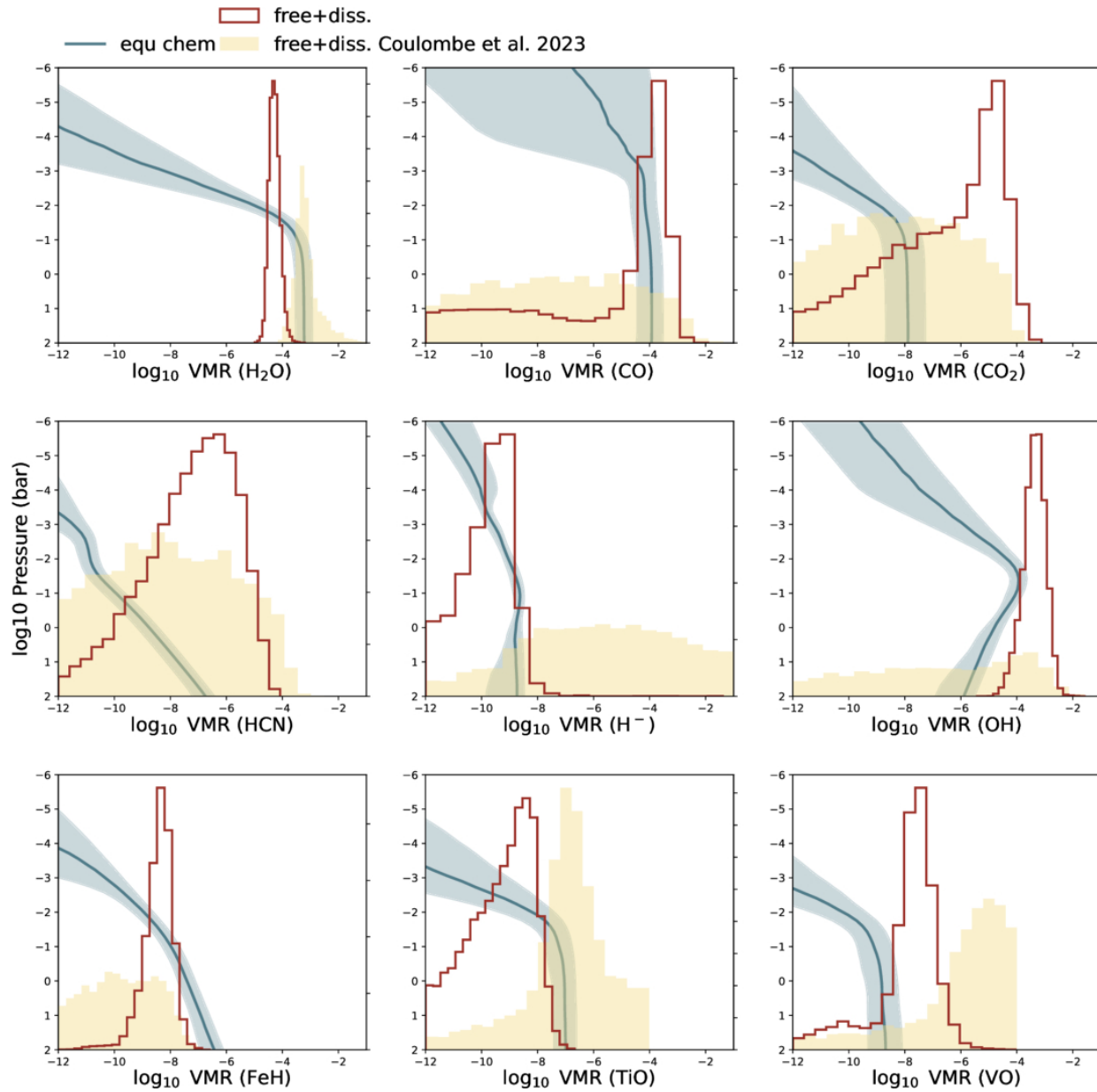
Figure 12. from Qinglin Ouyang et al 2026 Astrophys. J. 1004 doi:10.3847/1538-4357/ae736a https://dx.doi.org/10.3847/1538-4357/ae736a © 2026. The Author(s). Published by the American Astronomical Society.
