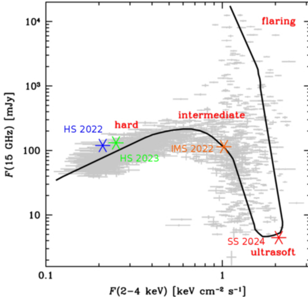
Figure 6. from Romana Mikušincová et al 2026 Astrophys. J. 1005 doi:10.3847/1538-4357/ae7366 https://dx.doi.org/10.3847/1538-4357/ae7366 © 2026. The Author(s). Published by the American Astronomical Society.
