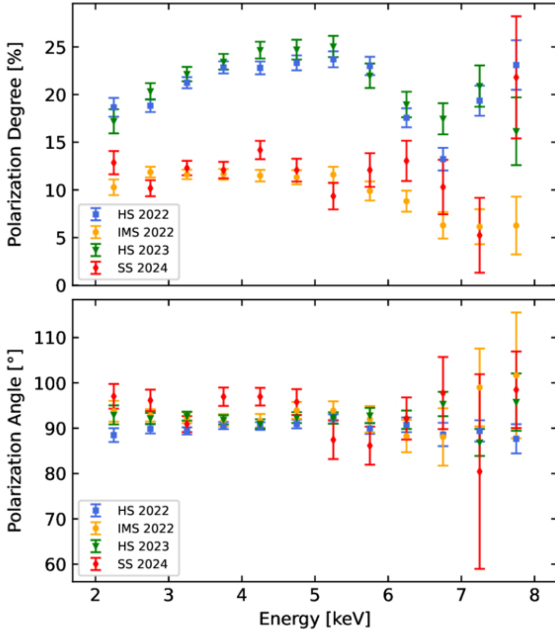
Figure 2. from Romana Mikušincová et al 2026 Astrophys. J. 1005 doi:10.3847/1538-4357/ae7366 https://dx.doi.org/10.3847/1538-4357/ae7366 © 2026. The Author(s). Published by the American Astronomical Society.
