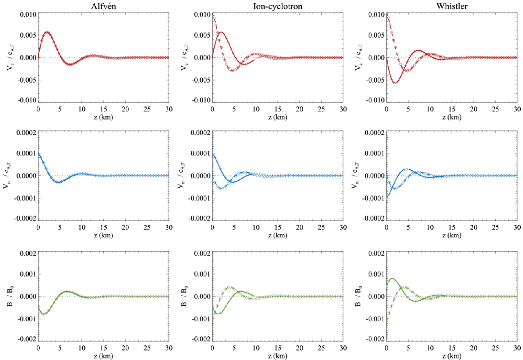
Figure 3. from David Martínez-Gómez 2026 Astrophys. J. 1004 doi:10.3847/1538-4357/ae7364 https://dx.doi.org/10.3847/1538-4357/ae7364 © 2026. The Author(s). Published by the American Astronomical Society.
