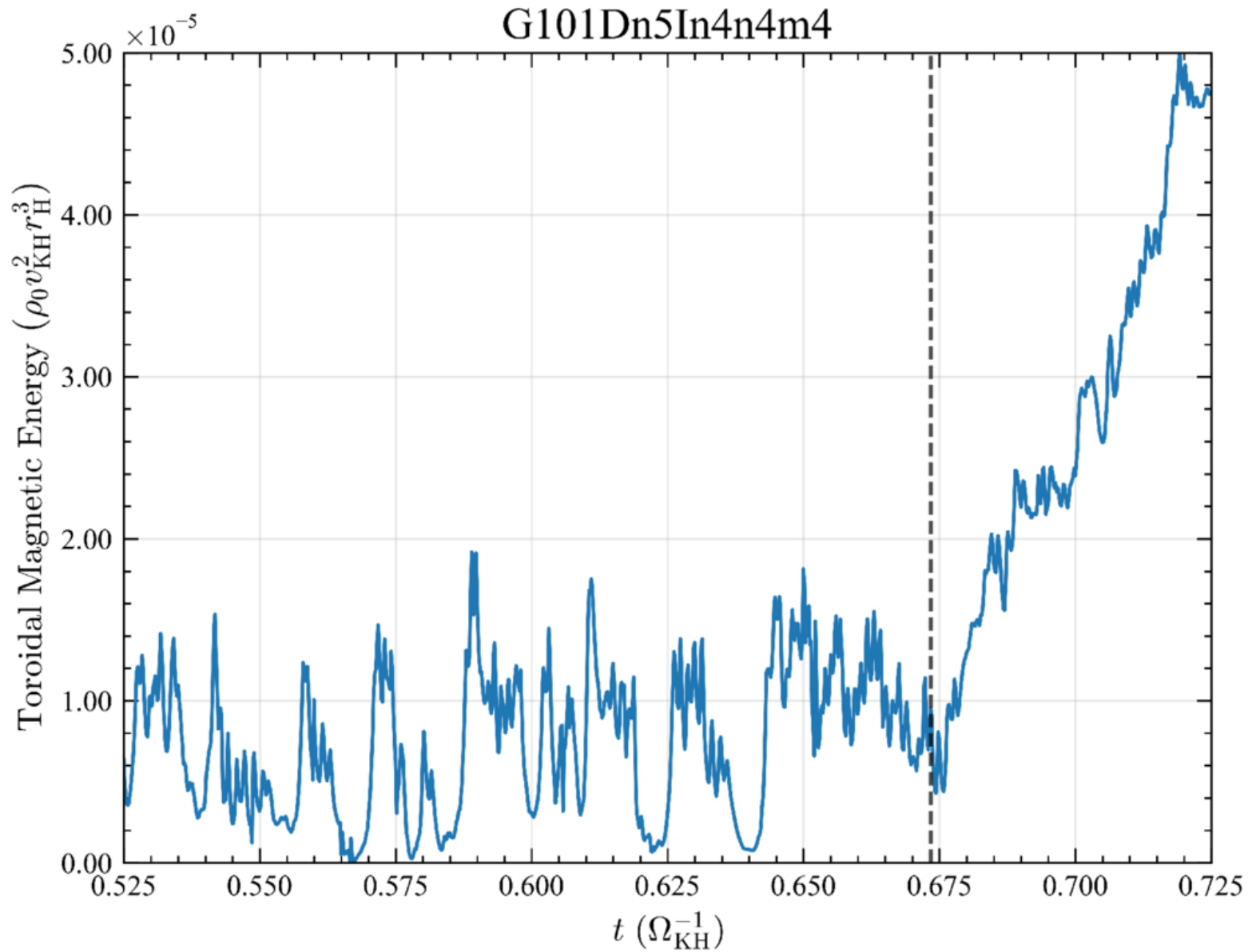
Figure 9. from Pengfei Tang et al 2026 Astrophys. J. 1005 doi:10.3847/1538-4357/ae733c https://dx.doi.org/10.3847/1538-4357/ae733c © 2026. The Author(s). Published by the American Astronomical Society.
