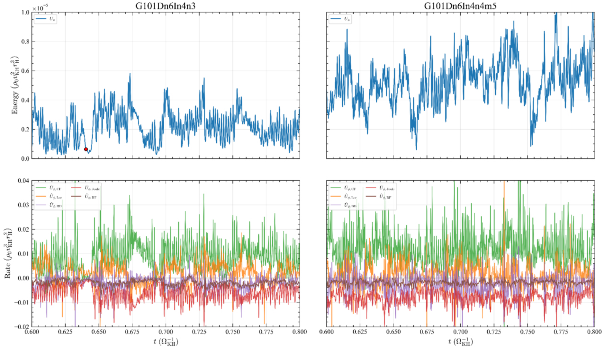
Figure 23. from Pengfei Tang et al 2026 Astrophys. J. 1005 doi:10.3847/1538-4357/ae733c https://dx.doi.org/10.3847/1538-4357/ae733c © 2026. The Author(s). Published by the American Astronomical Society.
