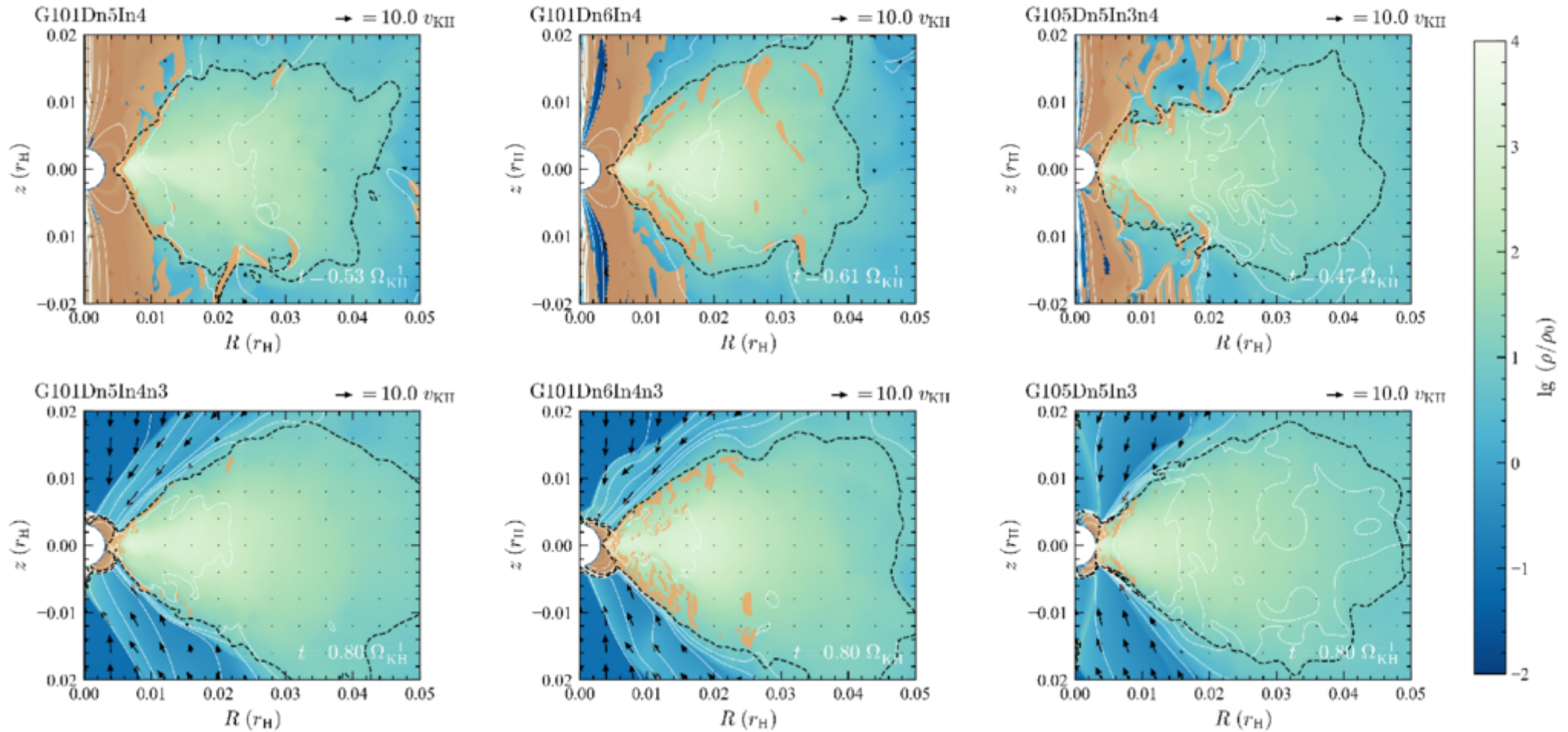
Figure 21. from Pengfei Tang et al 2026 Astrophys. J. 1005 doi:10.3847/1538-4357/ae733c https://dx.doi.org/10.3847/1538-4357/ae733c © 2026. The Author(s). Published by the American Astronomical Society.
