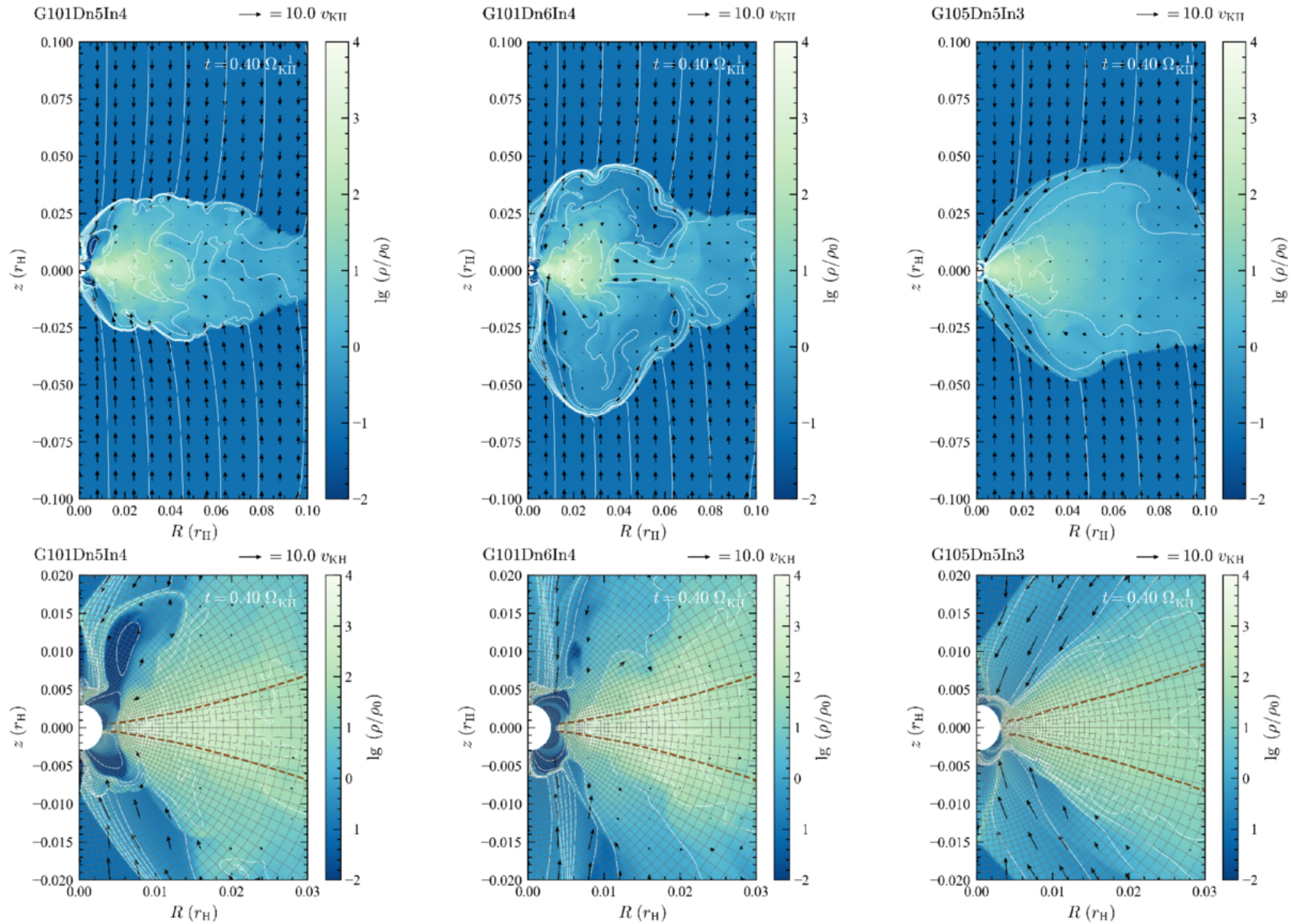
Figure 2. from Pengfei Tang et al 2026 Astrophys. J. 1005 doi:10.3847/1538-4357/ae733c https://dx.doi.org/10.3847/1538-4357/ae733c © 2026. The Author(s). Published by the American Astronomical Society.
