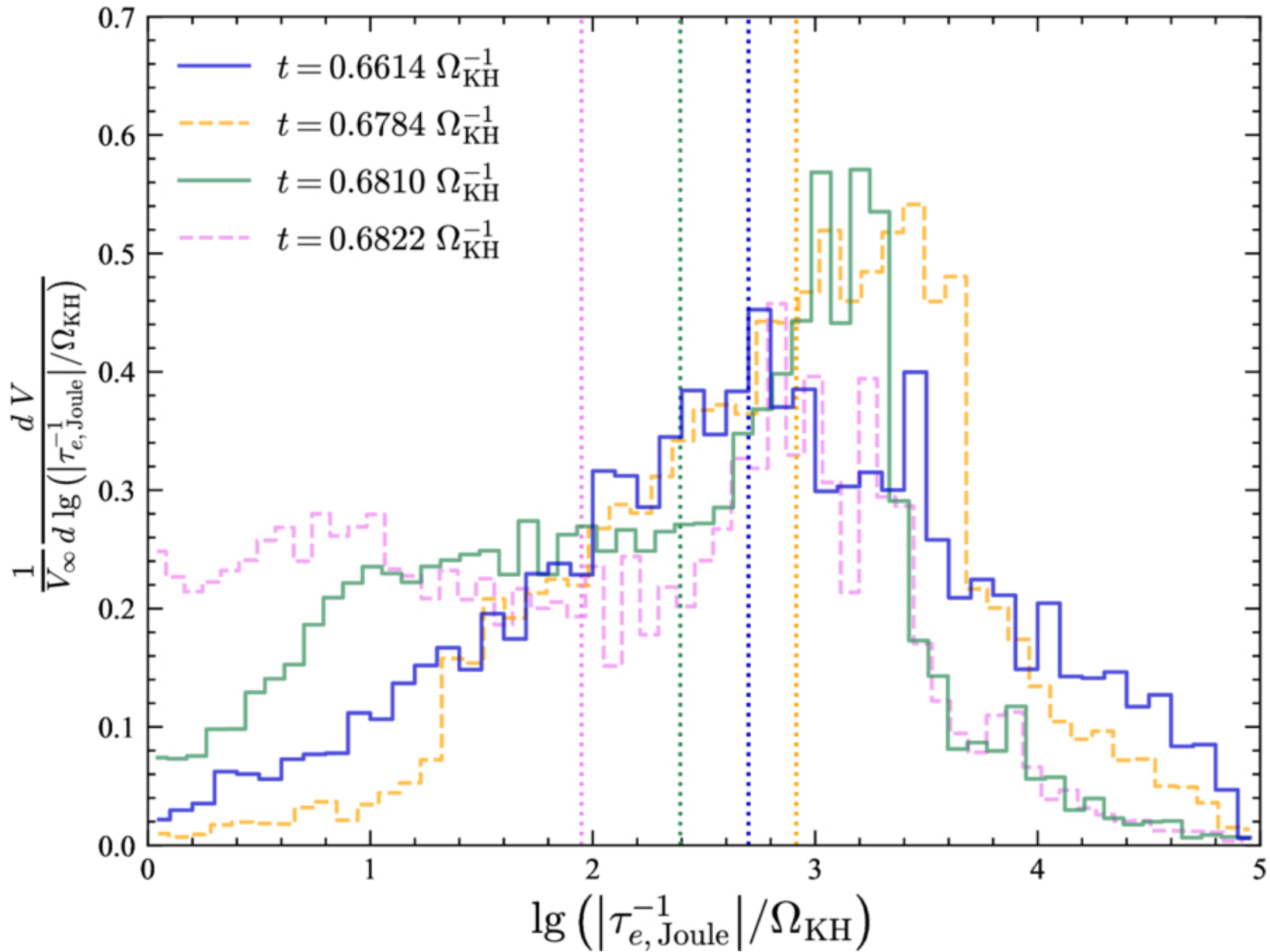
Figure 14. from Pengfei Tang et al 2026 Astrophys. J. 1005 doi:10.3847/1538-4357/ae733c https://dx.doi.org/10.3847/1538-4357/ae733c © 2026. The Author(s). Published by the American Astronomical Society.
