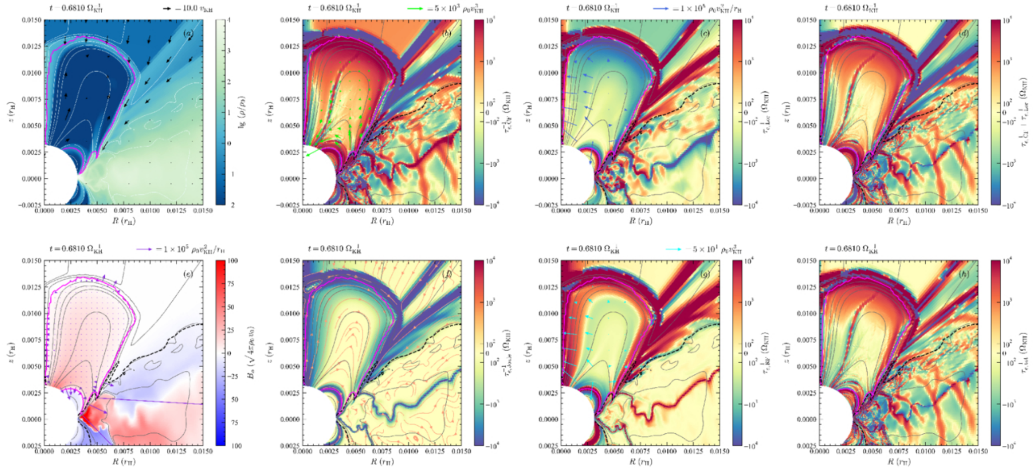
Figure 12. from Pengfei Tang et al 2026 Astrophys. J. 1005 doi:10.3847/1538-4357/ae733c https://dx.doi.org/10.3847/1538-4357/ae733c © 2026. The Author(s). Published by the American Astronomical Society.
