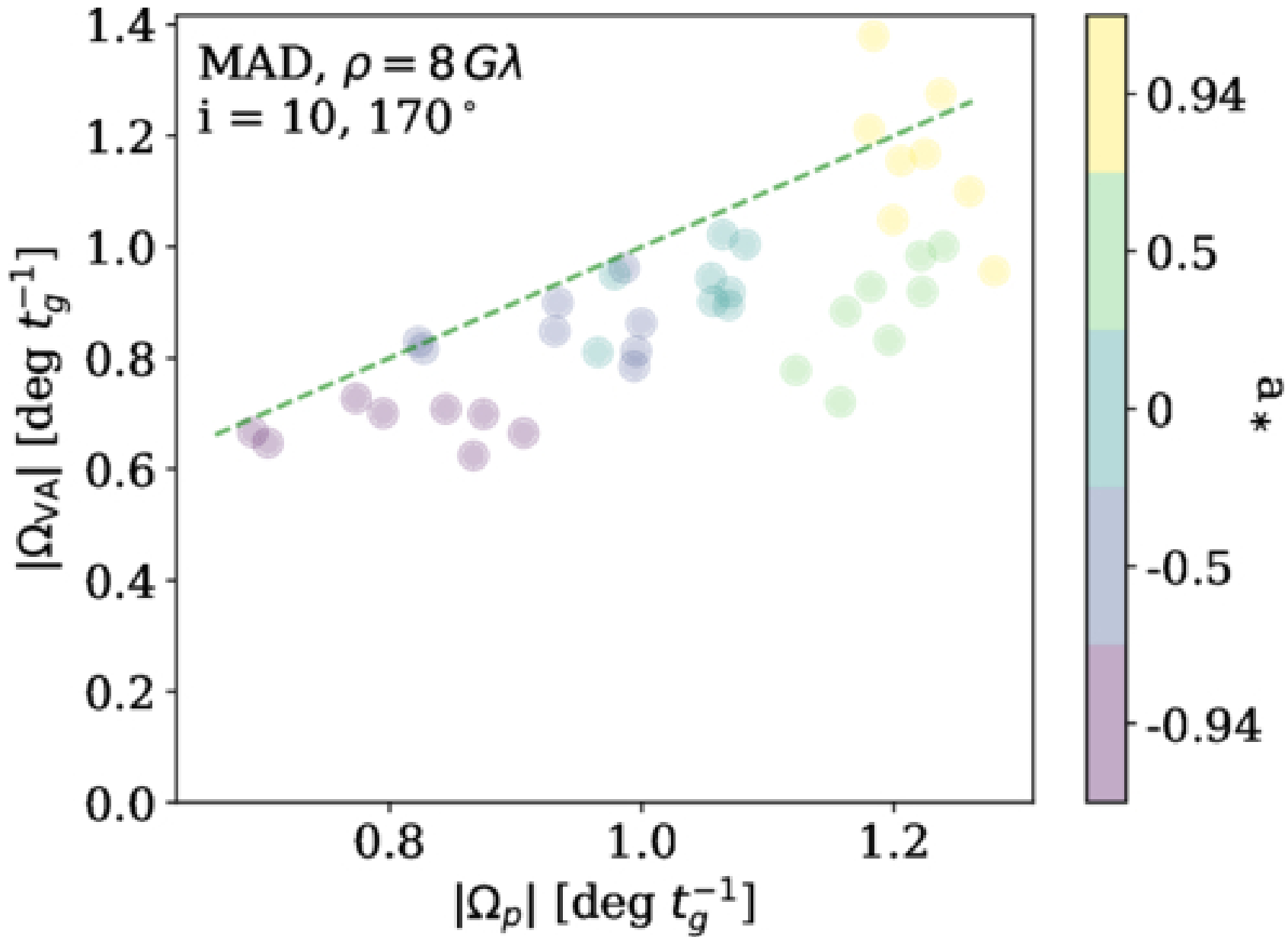
Figure 6. from Nicholas S. Conroy et al 2026 Astrophys. J. 1005 doi:10.3847/1538-4357/ae7326 https://dx.doi.org/10.3847/1538-4357/ae7326 © 2026. The Author(s). Published by the American Astronomical Society.
