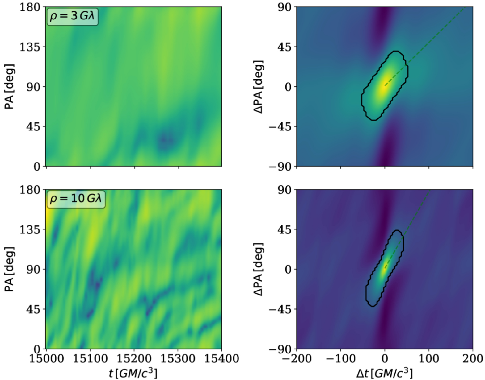
Figure 2. from Nicholas S. Conroy et al 2026 Astrophys. J. 1005 doi:10.3847/1538-4357/ae7326 https://dx.doi.org/10.3847/1538-4357/ae7326 © 2026. The Author(s). Published by the American Astronomical Society.
