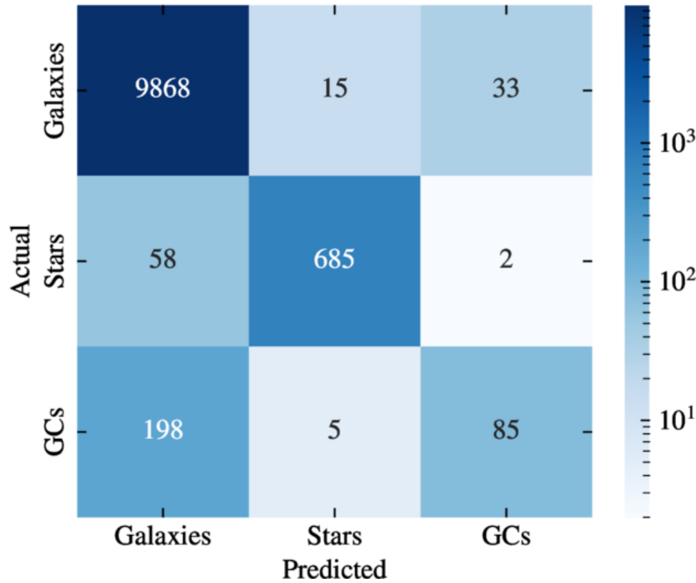
Confusion Matrix - Best RFC for 15 PCs input
