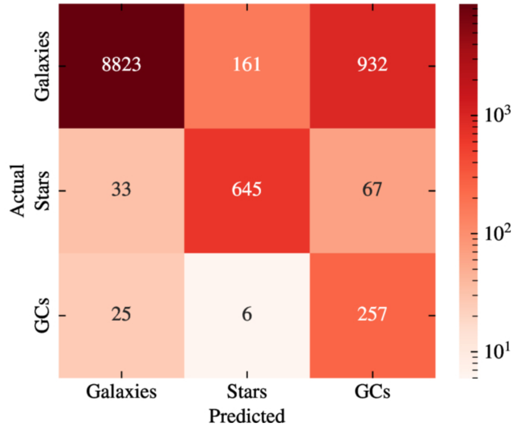
Confusion Matrix - Best MLPC for 15 PCs input
