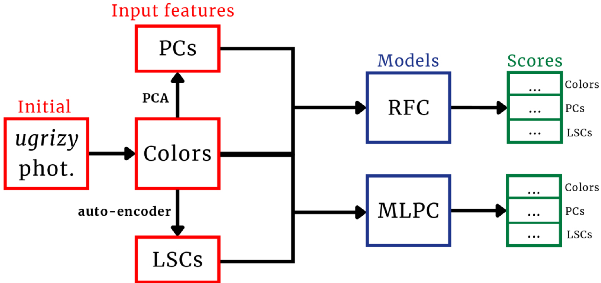
Figure 5. from Nicholas Schweder-Souza et al 2026 Astrophys. J. 1005 doi:10.3847/1538-4357/ae7321 https://dx.doi.org/10.3847/1538-4357/ae7321 © 2026. The Author(s). Published by the American Astronomical Society.
