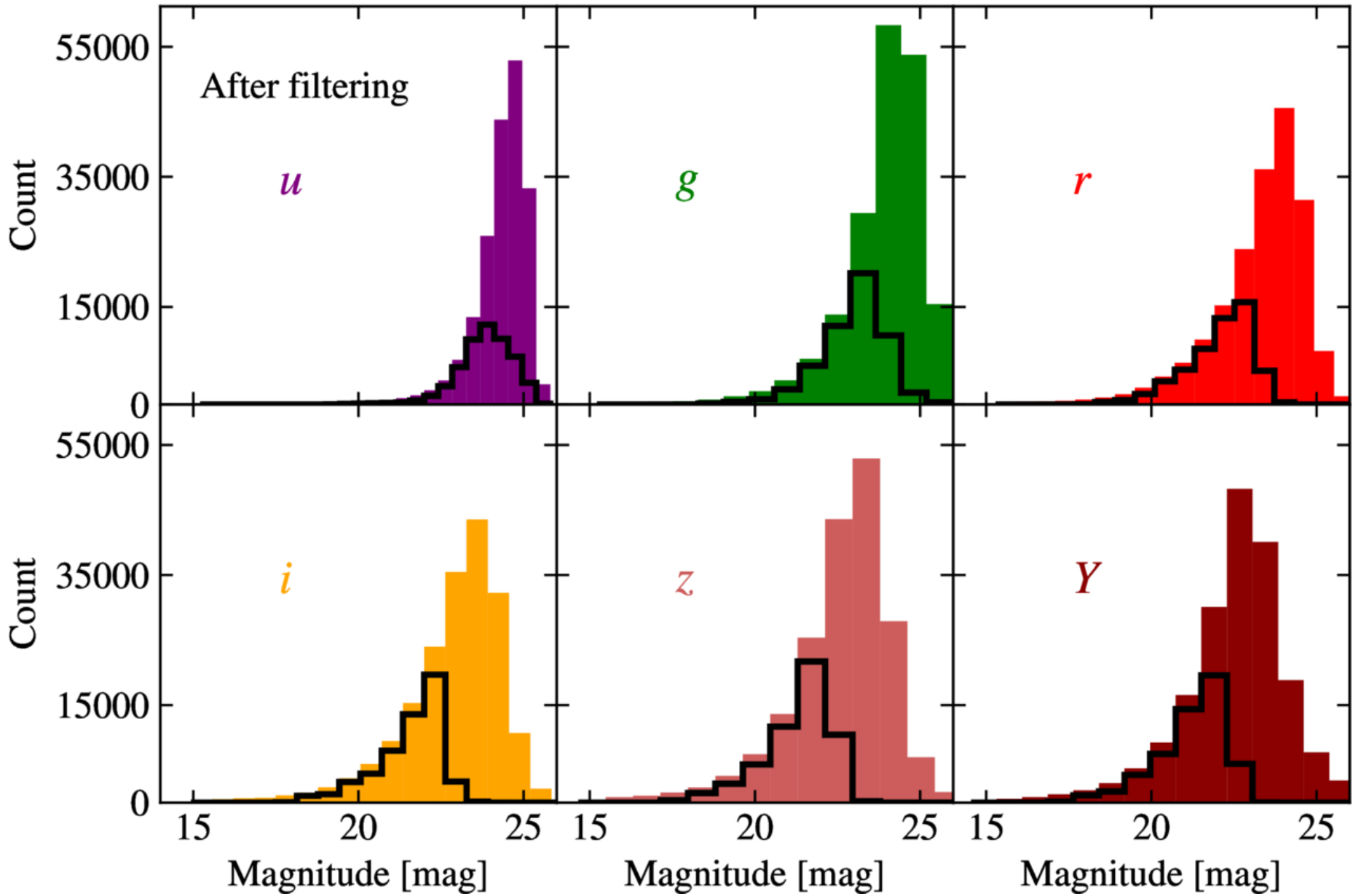
Figure 4. from Nicholas Schweder-Souza et al 2026 Astrophys. J. 1005 doi:10.3847/1538-4357/ae7321 https://dx.doi.org/10.3847/1538-4357/ae7321 © 2026. The Author(s). Published by the American Astronomical Society.
