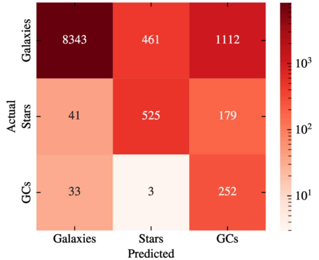
Confusion Matrix - Best MLPC for 2 LSCs input
