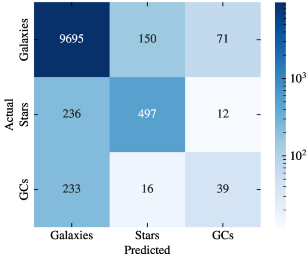
Confusion Matrix - Best RFC for 2 LSCs input
