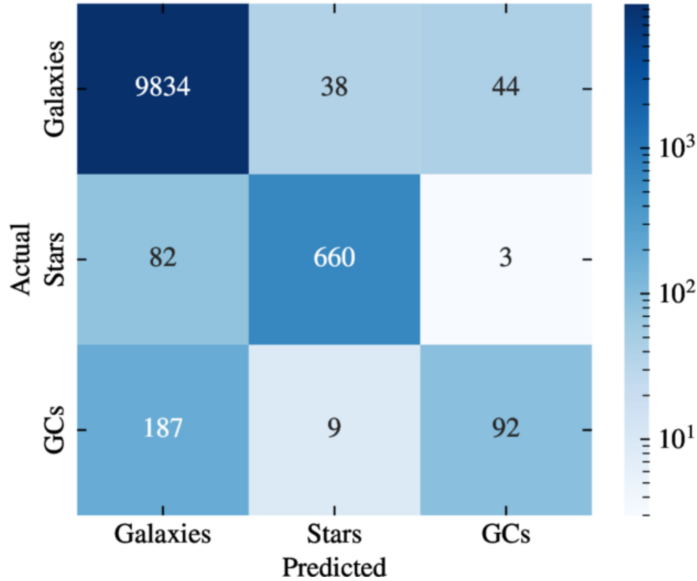
Confusion Matrix - Best RFC for 4 LSCs input
