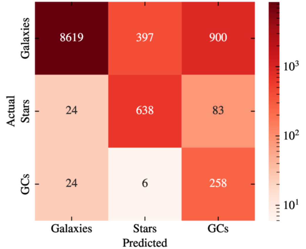
Confusion Matrix - Best MLPC for 4 LSCs input
