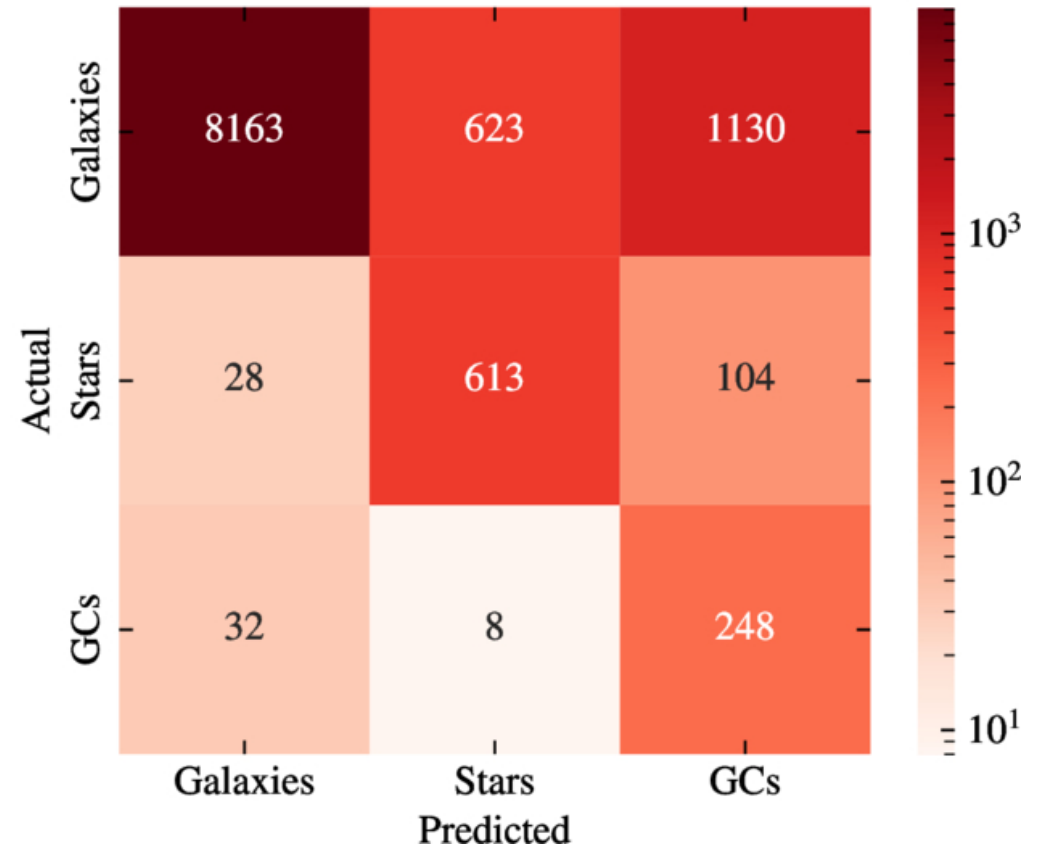
Confusion Matrix - Best MLPC for 2 PCs input
