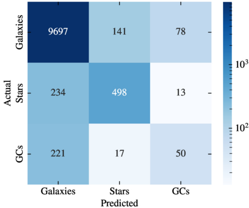
Confusion Matrix - Best RFC for 2 PCs input
