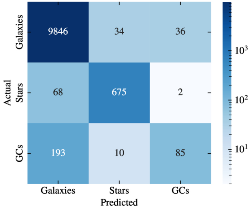
Confusion Matrix - Best RFC for 4 PCs input
