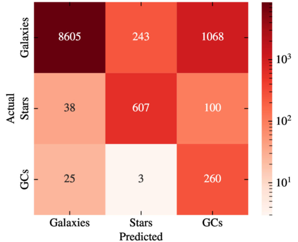
Confusion Matrix - Best MLPC for 4 PCs input
