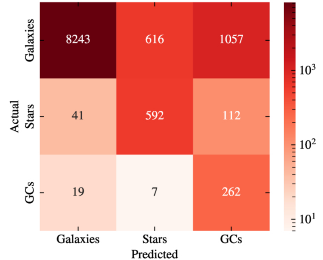
Confusion Matrix - Best MLPC for 2 Colors input
