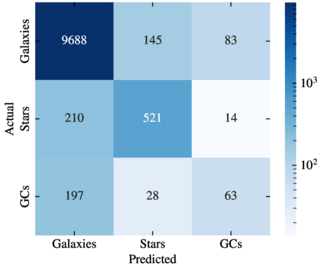
Confusion Matrix - Best RFC for 2 Colors input
