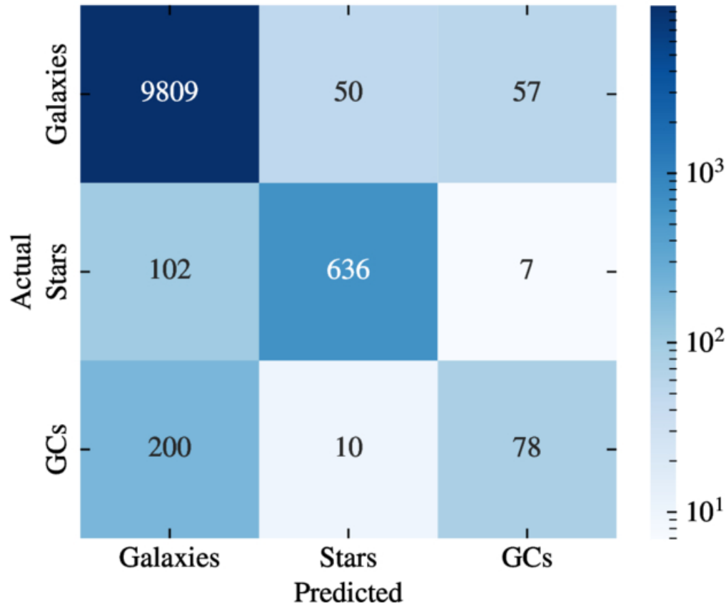
Confusion Matrix - Best RFC for 4 Colors input
