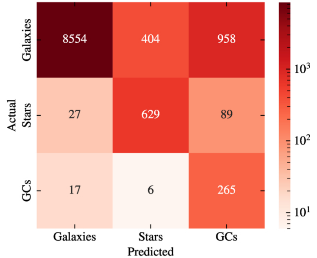
Confusion Matrix - Best MLPC for 4 Colors input
