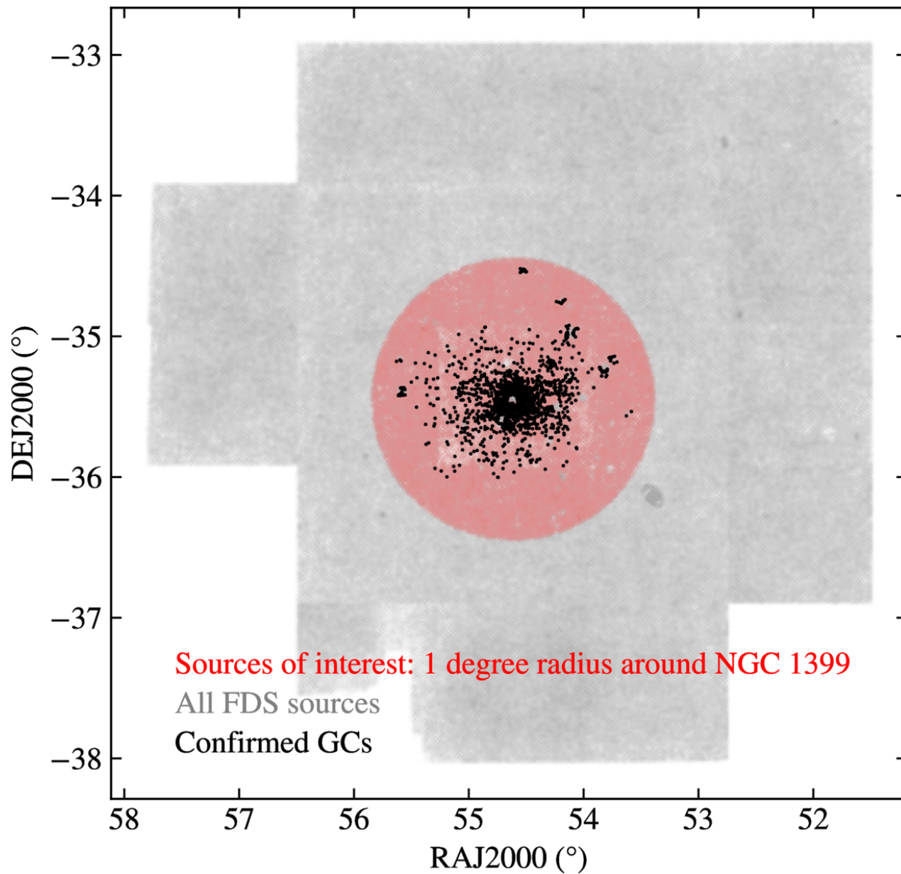
Figure 1. from Nicholas Schweder-Souza et al 2026 Astrophys. J. 1005 doi:10.3847/1538-4357/ae7321 https://dx.doi.org/10.3847/1538-4357/ae7321 © 2026. The Author(s). Published by the American Astronomical Society.
